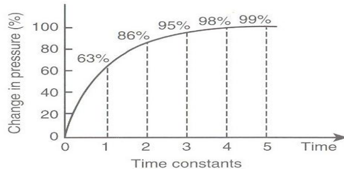
Gambar 1. Time Constant 2
